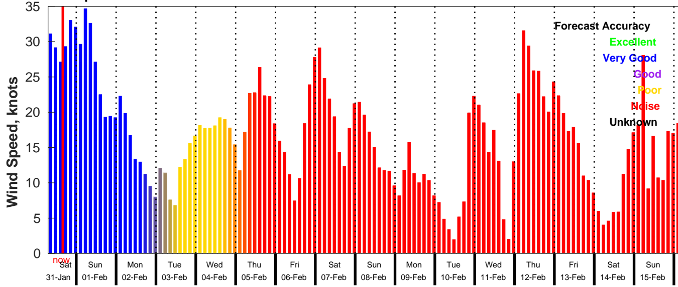
GFS Wind Speed Forecast for NDBC 41013 from 31-Jan-2026 07:00:00 to 16-Feb-2026 07:00:00
