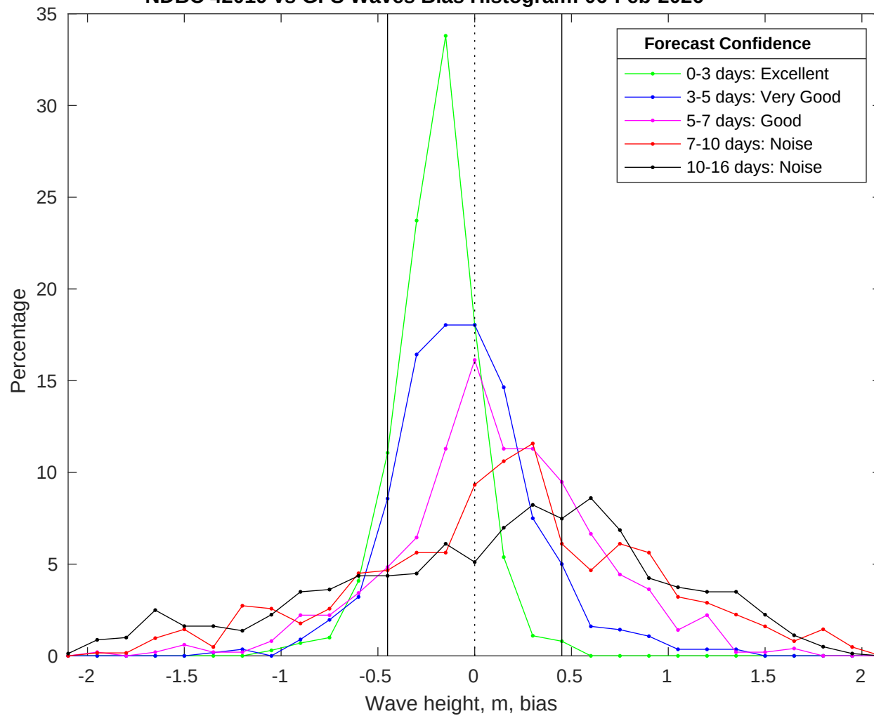
NDBC 42019 vs GFS Waves Bias Histogram: 06-Feb-2026
