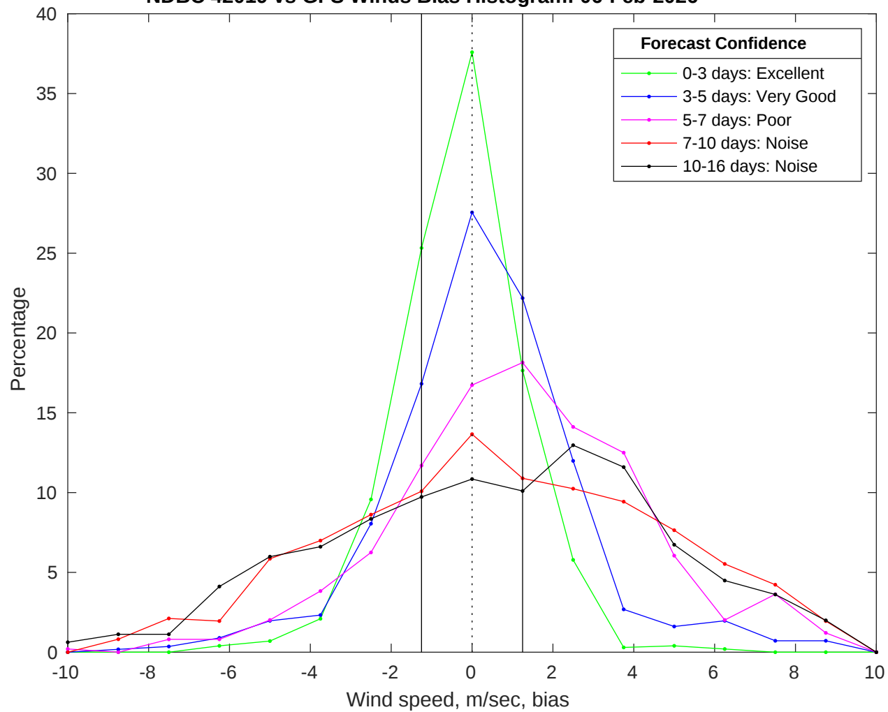
NDBC 42019 vs GFS Winds Bias Histogram: 06-Feb-2026
