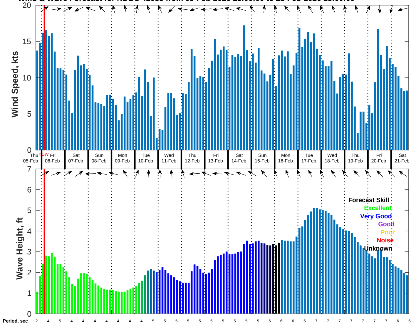
Wind & Wave Forecast for NDBC 42035 from 05-Feb-2026 18:00:00 to 21-Feb-2026 18:00:00
