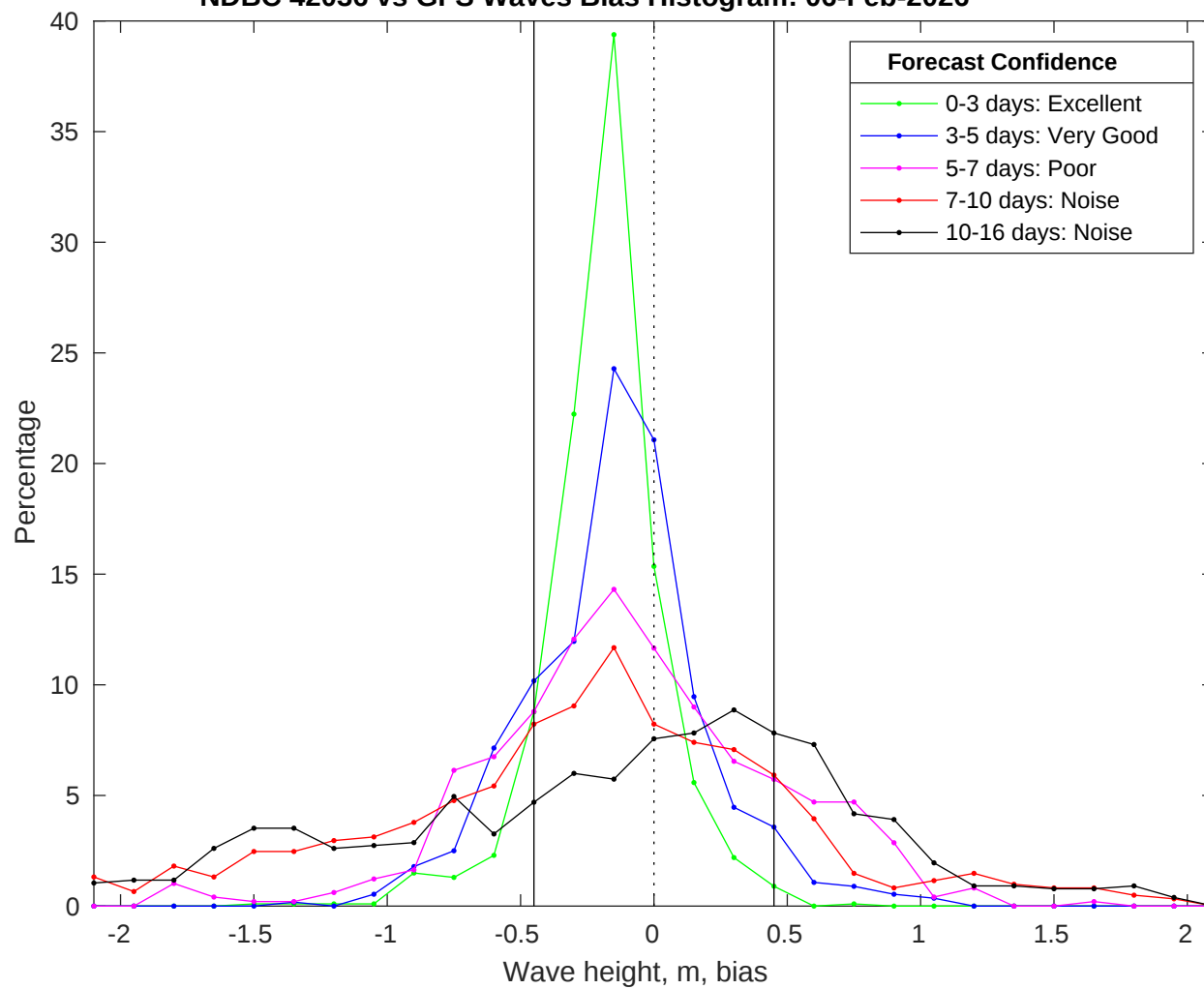
NDBC 42036 vs GFS Waves Bias Histogram: 06-Feb-2026
