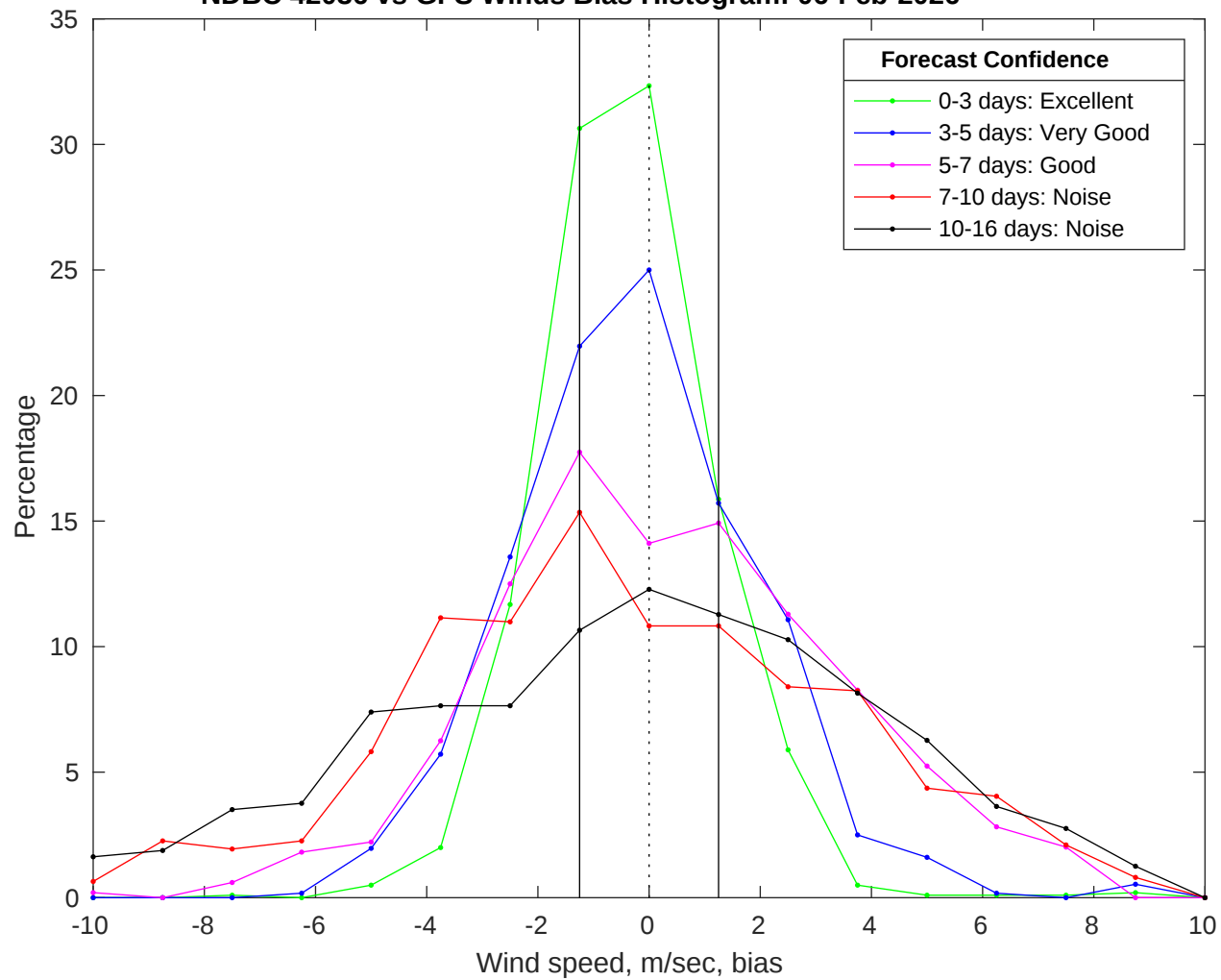
NDBC 42036 vs GFS Winds Bias Histogram: 06-Feb-2026
