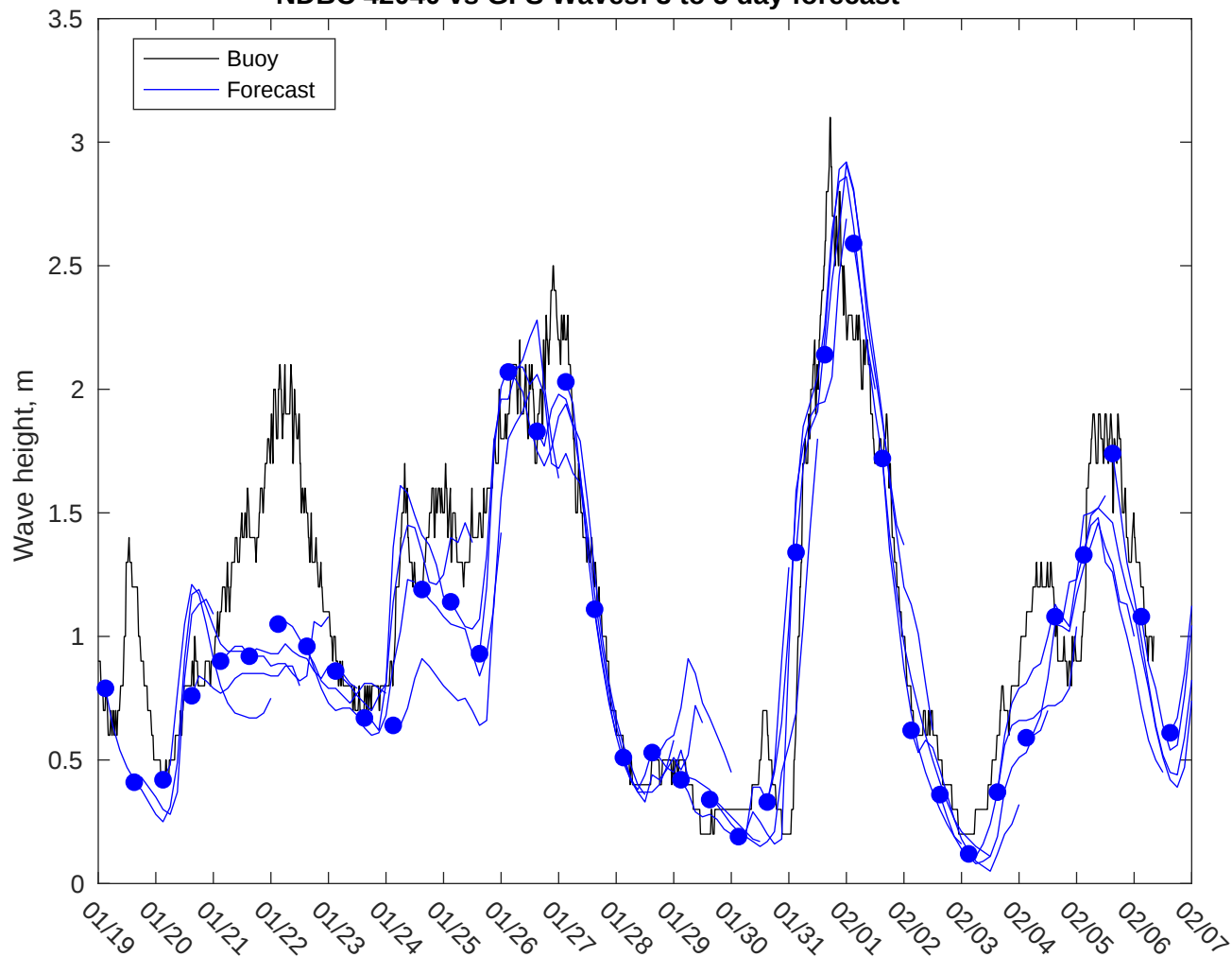
NDBC 42040 vs GFS Waves: 3 to 5 day forecast
