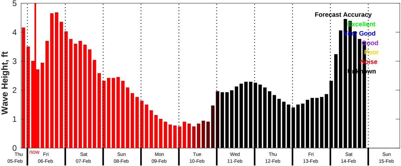
CMEMS Wave Forecast for NDBC 42058 from 05-Feb-2026 20:00:00 to 15-Feb-2026 20:00:00
