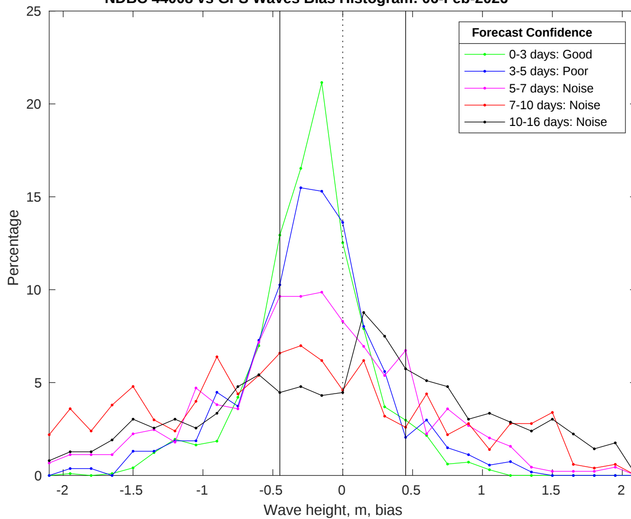
NDBC 44008 vs GFS Waves Bias Histogram: 06-Feb-2026
