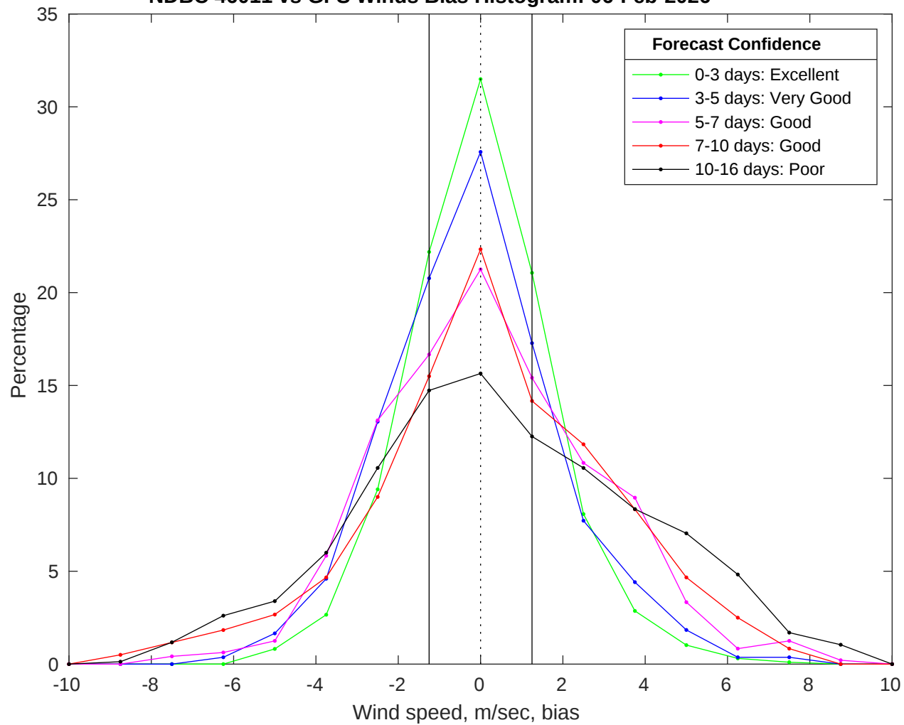
NDBC 46011 vs GFS Winds Bias Histogram: 06-Feb-2026
