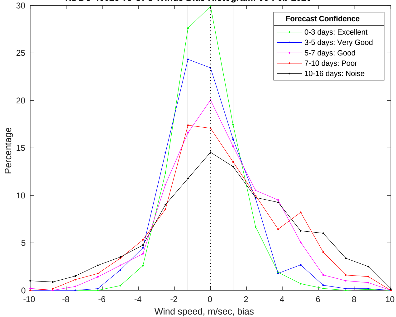
NDBC 46028 vs GFS Winds Bias Histogram: 06-Feb-2026
