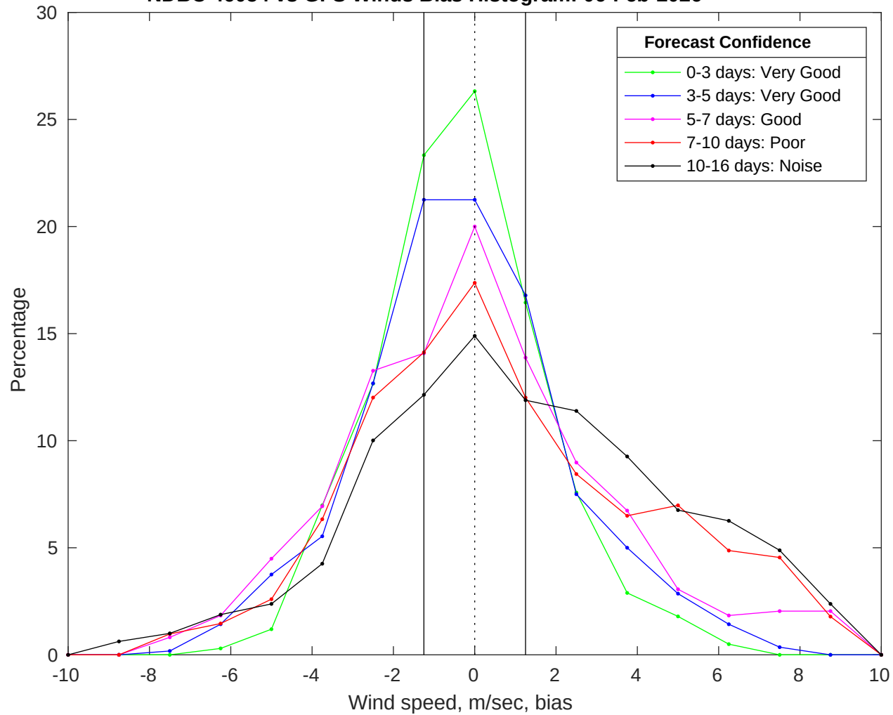
NDBC 46054 vs GFS Winds Bias Histogram: 06-Feb-2026
