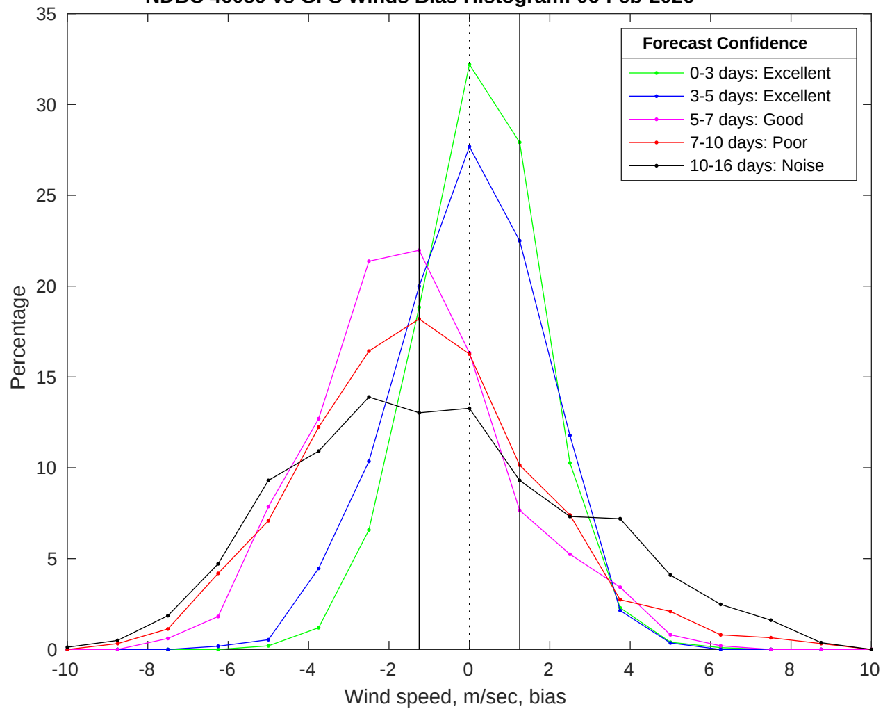
NDBC 46059 vs GFS Winds Bias Histogram: 06-Feb-2026
