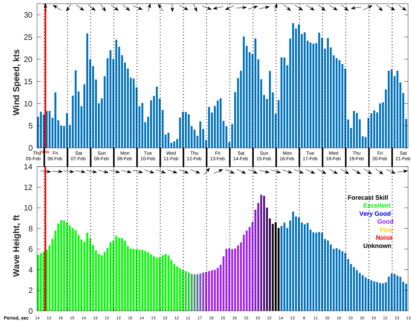
Wind & Wave Forecast for NDBC 46069 from 05-Feb-2026 16:00:00 to 21-Feb-2026 16:00:00
