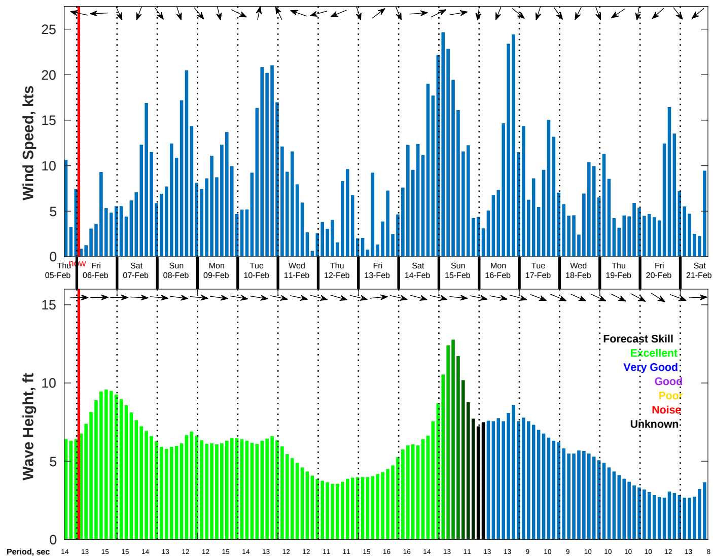
Wind & Wave Forecast for NDBC 46215 from 05-Feb-2026 16:00:00 to 21-Feb-2026 16:00:00
