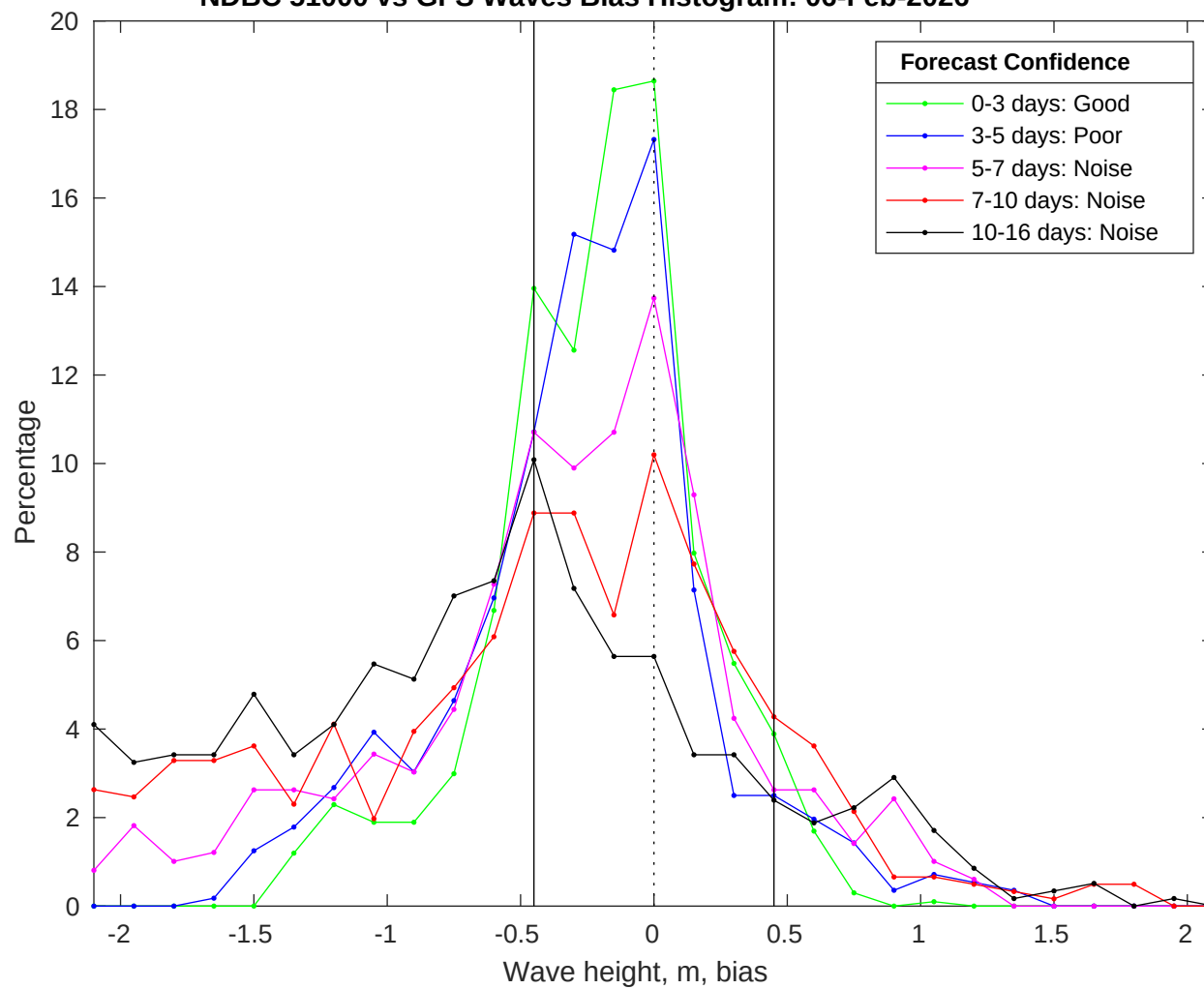
NDBC 51000 vs GFS Waves Bias Histogram: 06-Feb-2026
