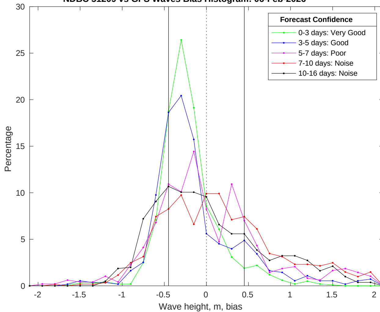
NDBC 51209 vs GFS Waves Bias Histogram: 06-Feb-2026
