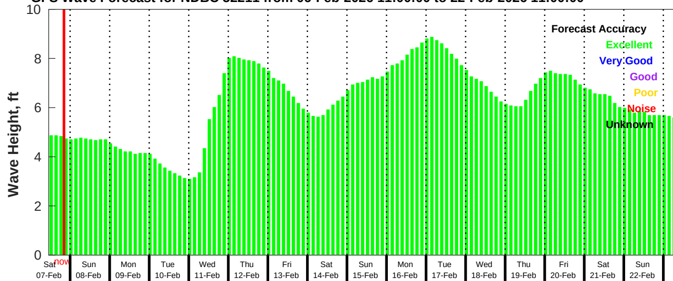
GFS Wave Forecast for NDBC 52211 from 06-Feb-2026 11:00:00 to 22-Feb-2026 11:00:00
