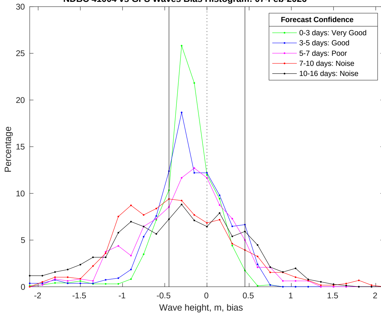
NDBC 41004 vs GFS Waves Bias Histogram: 07-Feb-2026
