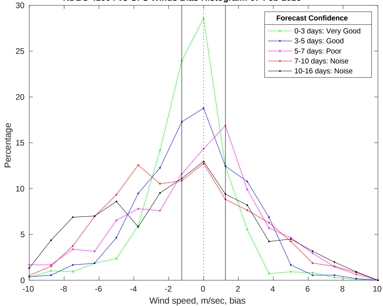
NDBC 41004 vs GFS Winds Bias Histogram: 07-Feb-2026
