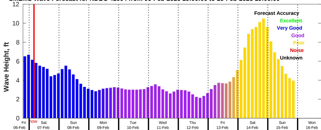
CMEMS Wave Forecast for NDBC 41004 from 06-Feb-2026 19:00:00 to 16-Feb-2026 19:00:00
