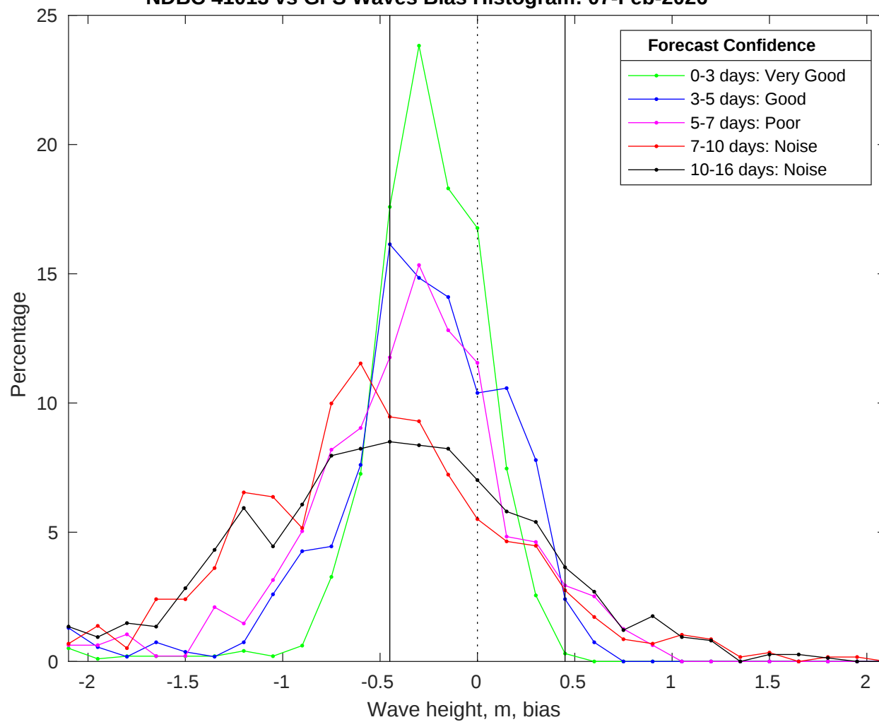
NDBC 41013 vs GFS Waves Bias Histogram: 07-Feb-2026
