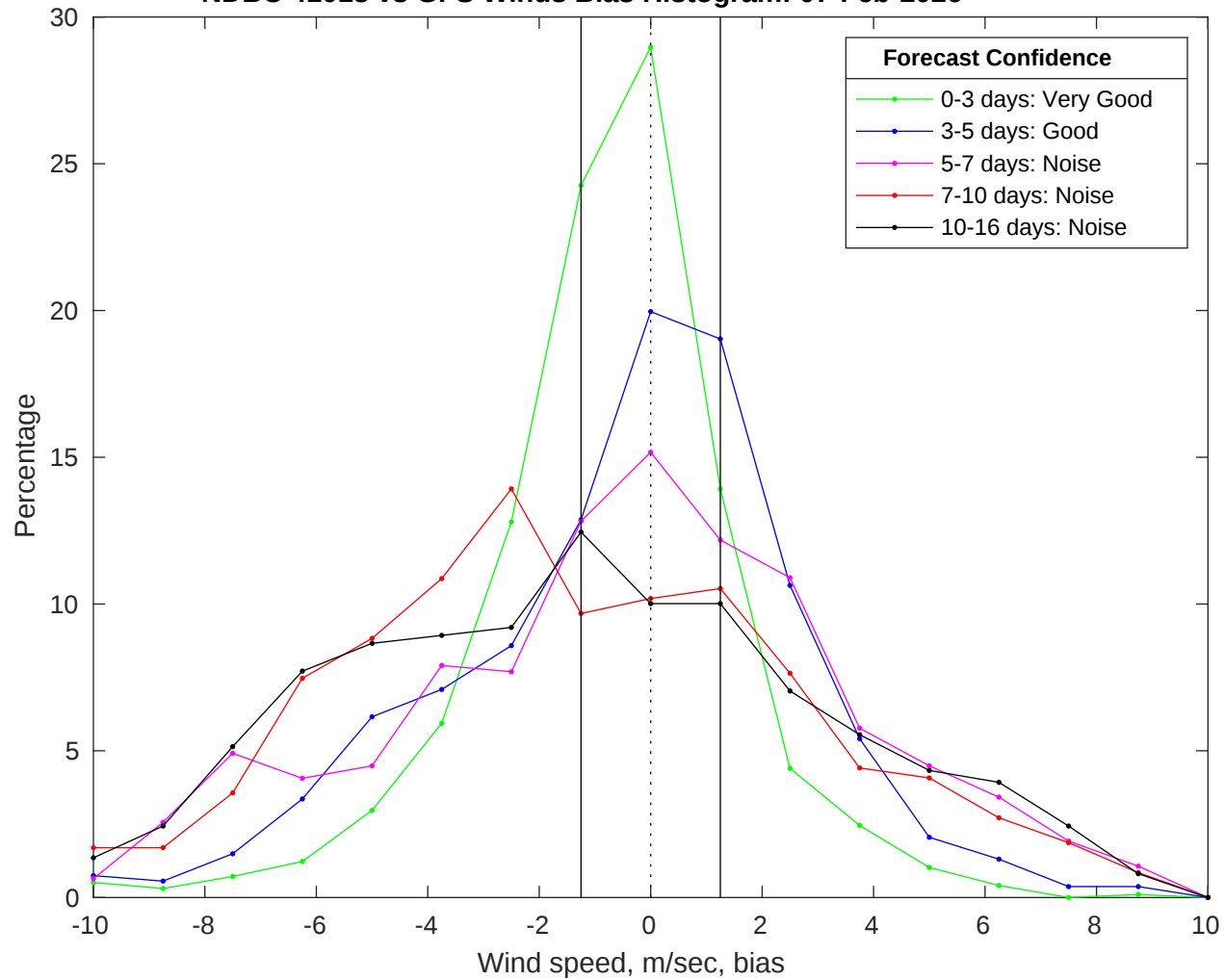
NDBC 41013 vs GFS Winds Bias Histogram: 07-Feb-2026
