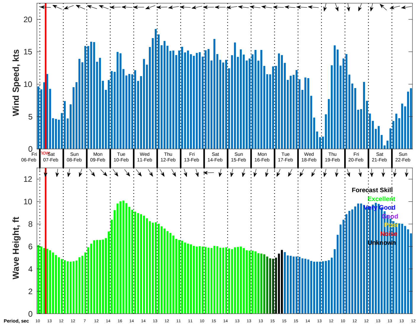
Wind & Wave Forecast for NDBC 41040 from 06-Feb-2026 21:00:00 to 22-Feb-2026 21:00:00
