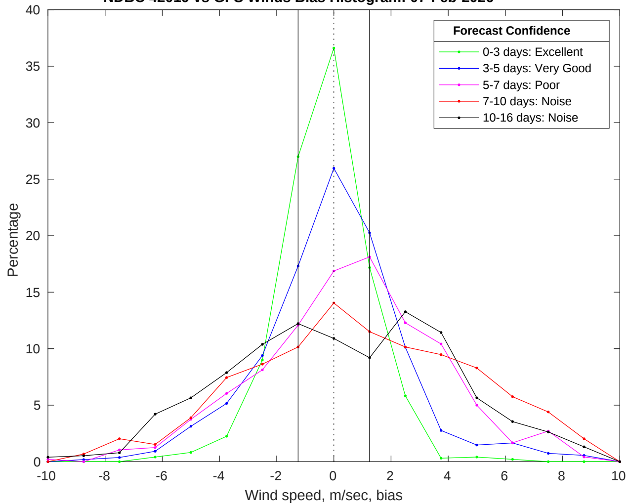
NDBC 42019 vs GFS Winds Bias Histogram: 07-Feb-2026
