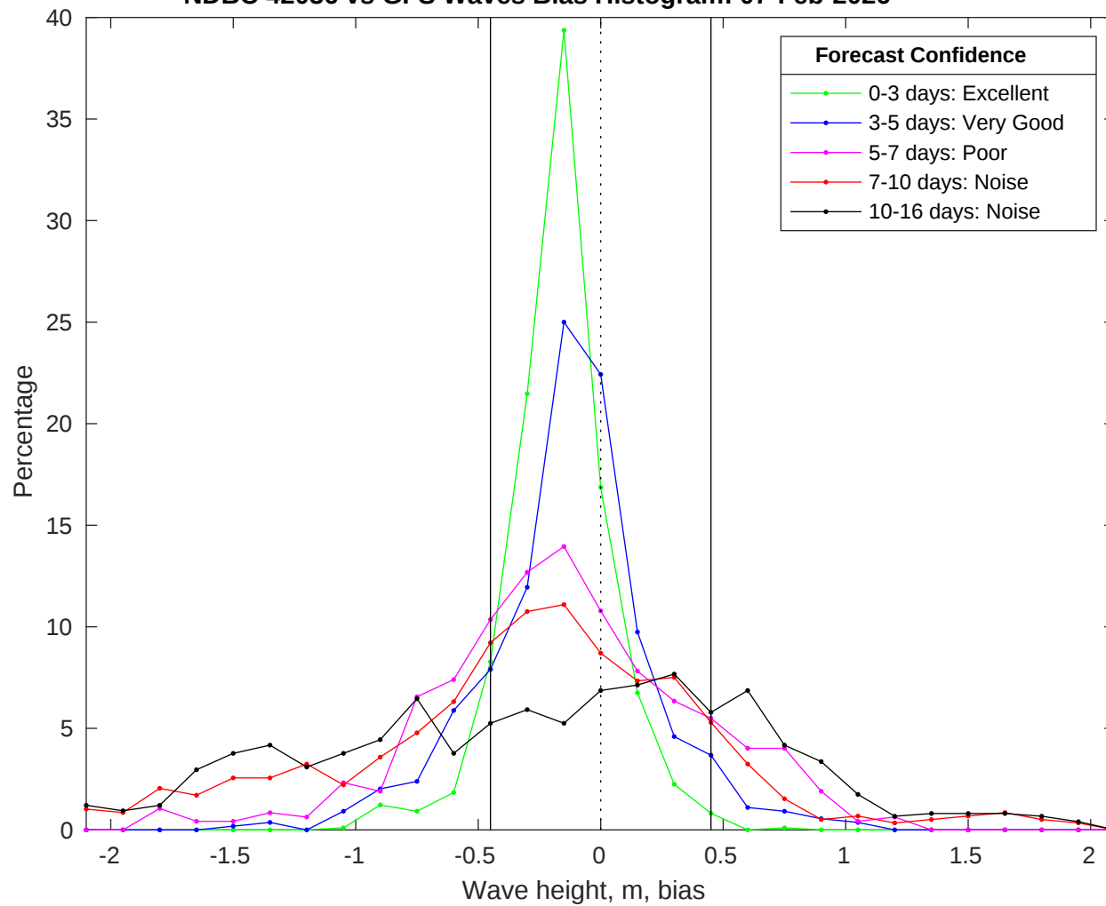
NDBC 42036 vs GFS Waves Bias Histogram: 07-Feb-2026
