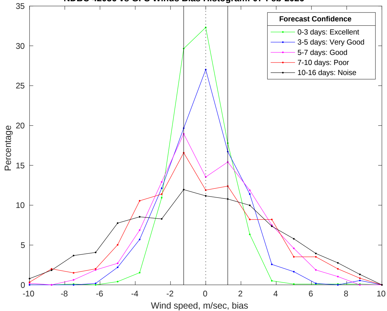
NDBC 42036 vs GFS Winds Bias Histogram: 07-Feb-2026
