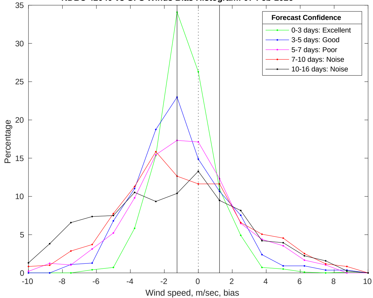
NDBC 42040 vs GFS Winds Bias Histogram: 07-Feb-2026
