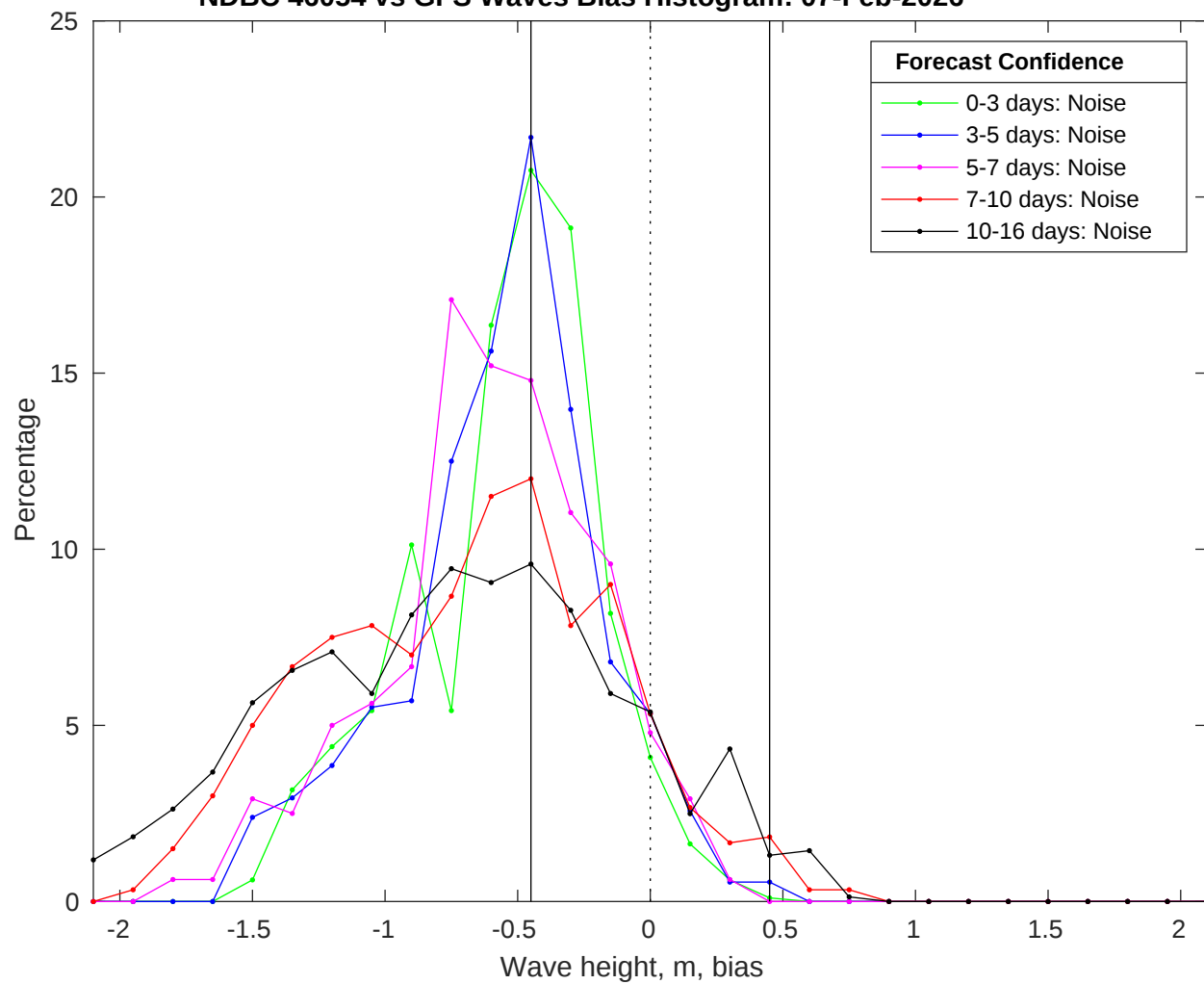
NDBC 46054 vs GFS Waves Bias Histogram: 07-Feb-2026
