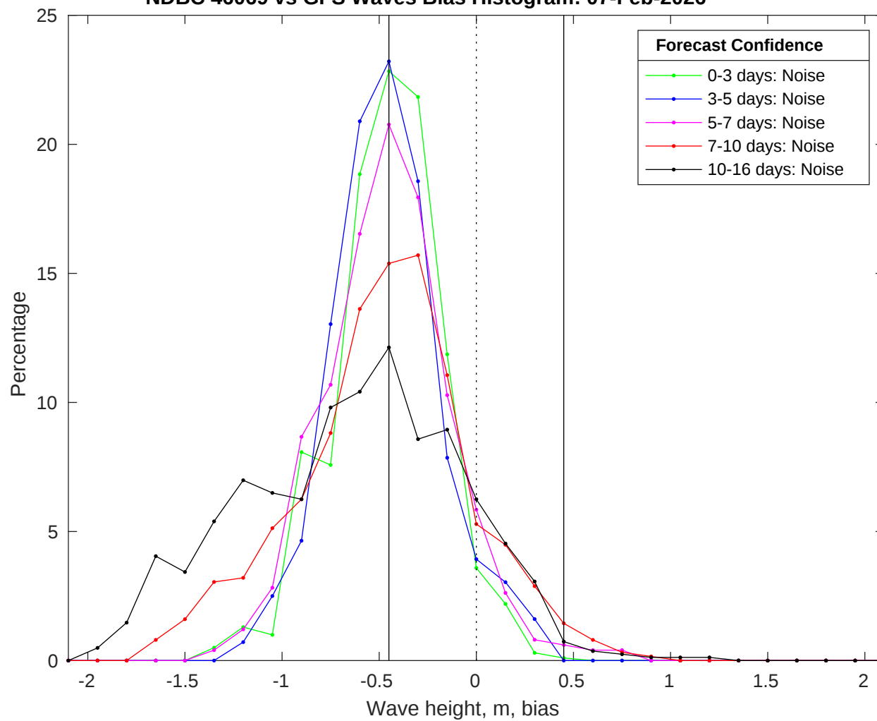
NDBC 46069 vs GFS Waves Bias Histogram: 07-Feb-2026
