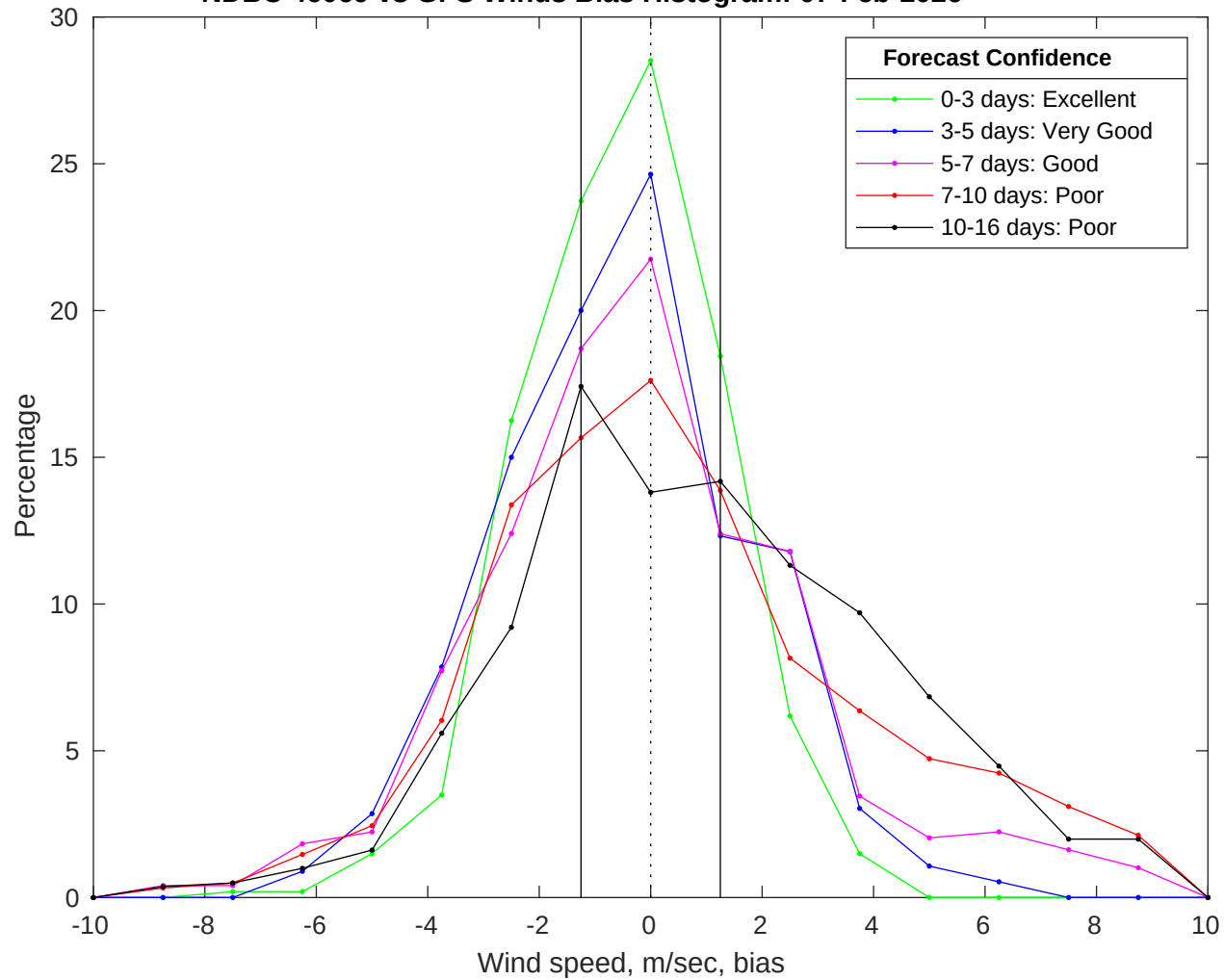
NDBC 46069 vs GFS Winds Bias Histogram: 07-Feb-2026
