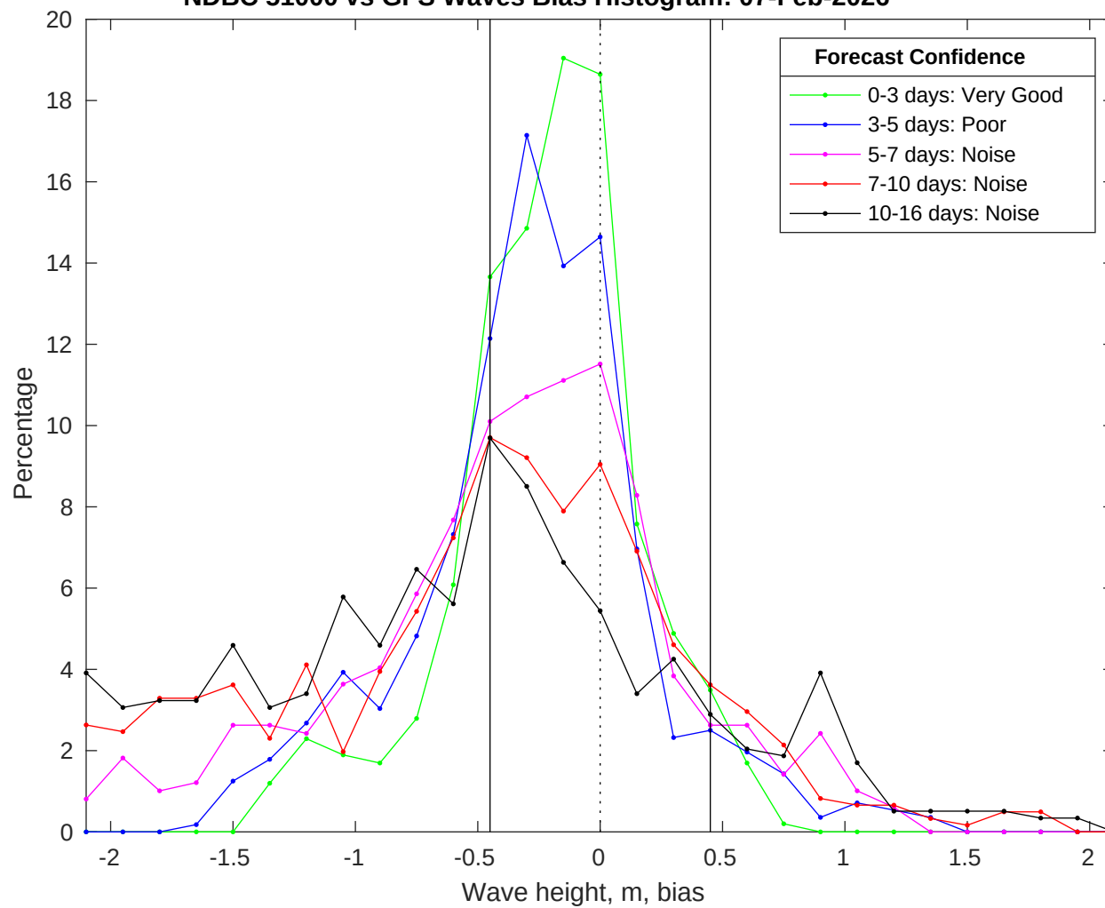
NDBC 51000 vs GFS Waves Bias Histogram: 07-Feb-2026
