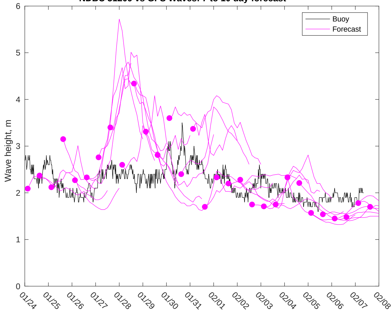
NDBC 51209 vs GFS Waves: 7 to 10 day forecast
