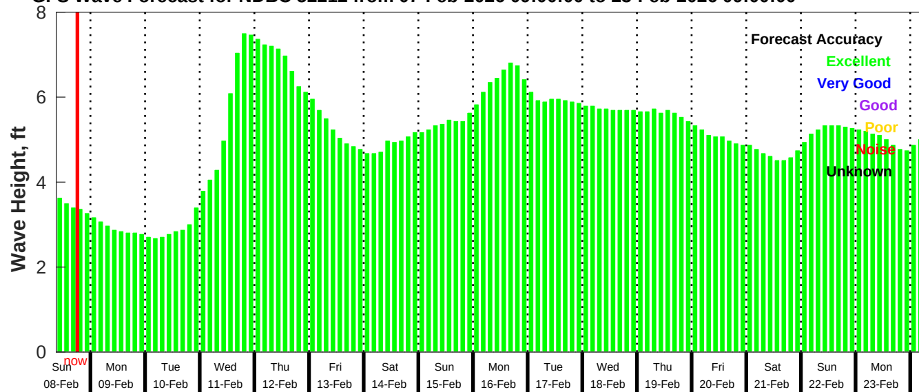
GFS Wave Forecast for NDBC 52212 from 07-Feb-2026 09:00:00 to 23-Feb-2026 09:00:00
