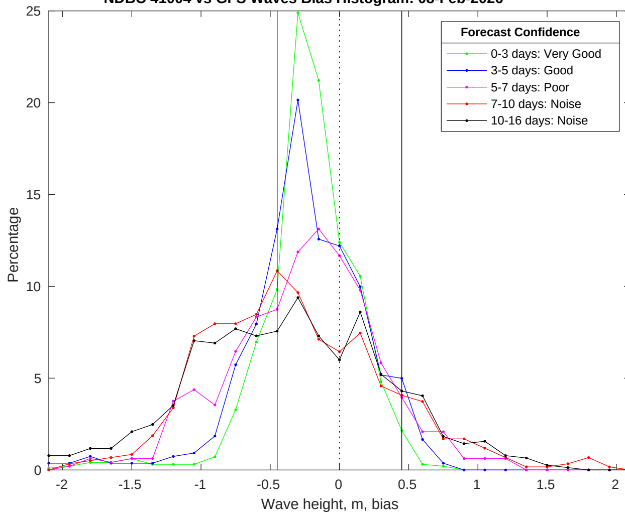
NDBC 41004 vs GFS Waves Bias Histogram: 08-Feb-2026
