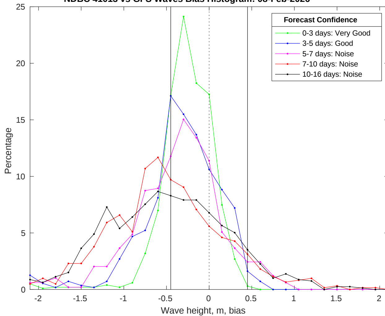
NDBC 41013 vs GFS Waves Bias Histogram: 08-Feb-2026
