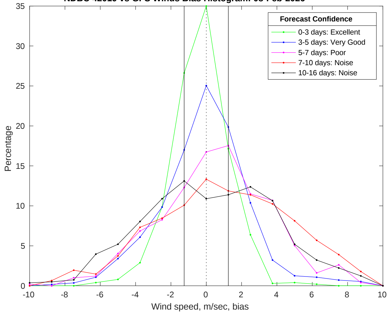
NDBC 42019 vs GFS Winds Bias Histogram: 08-Feb-2026
