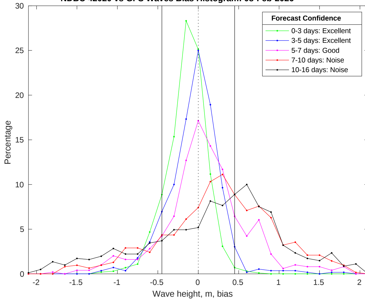
NDBC 42020 vs GFS Waves Bias Histogram: 08-Feb-2026
