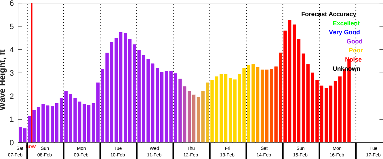
CMEMS Wave Forecast for NDBC 42020 from 07-Feb-2026 18:00:00 to 17-Feb-2026 18:00:00
