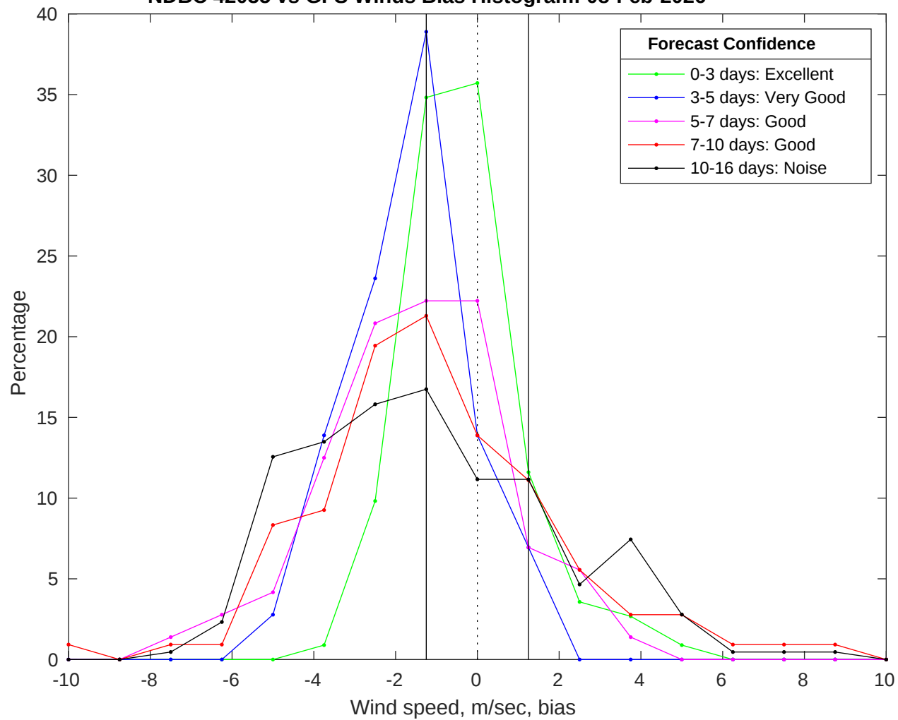
NDBC 42035 vs GFS Winds Bias Histogram: 08-Feb-2026
