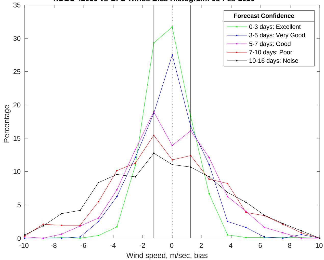
NDBC 42036 vs GFS Winds Bias Histogram: 08-Feb-2026
