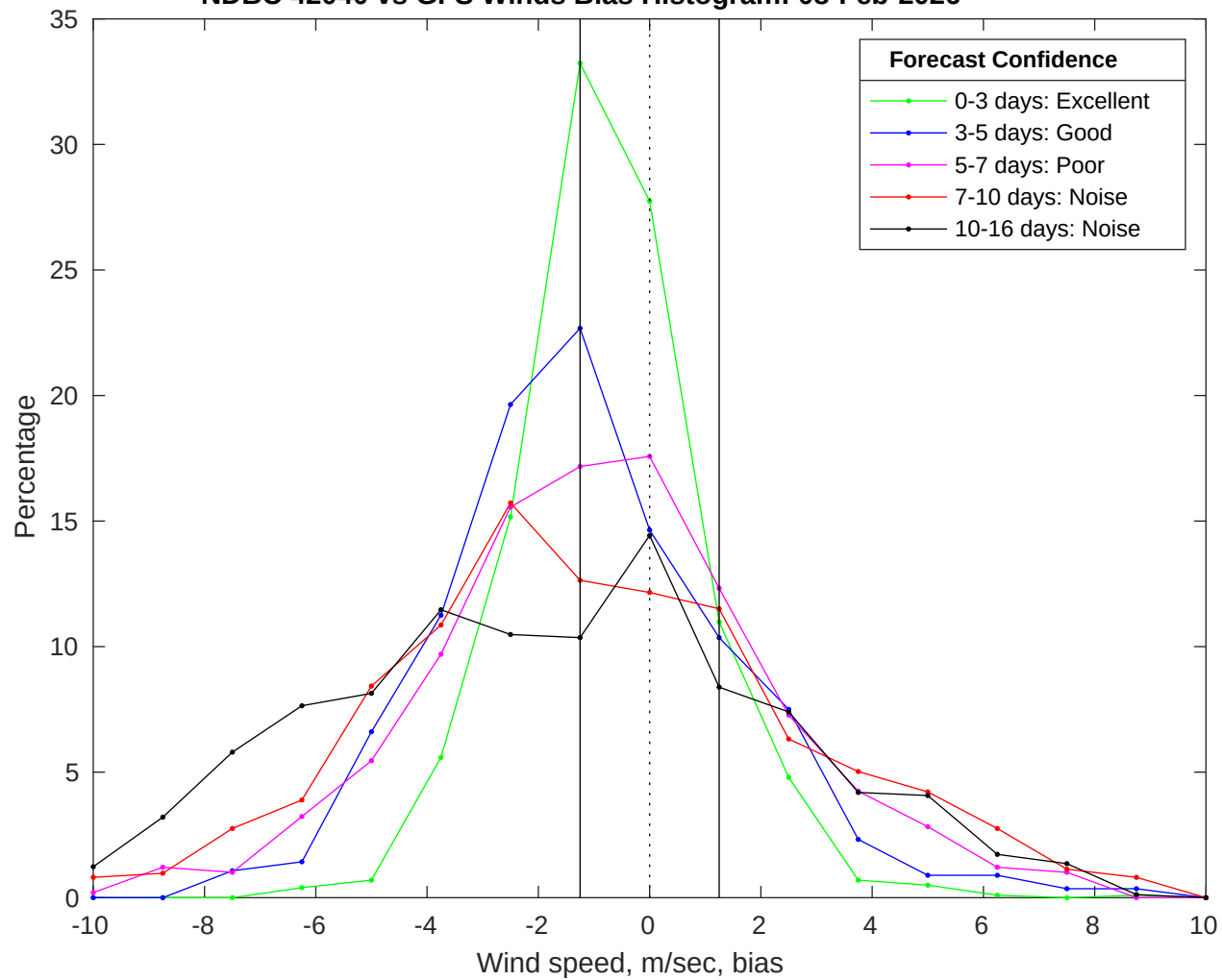
NDBC 42040 vs GFS Winds Bias Histogram: 08-Feb-2026
