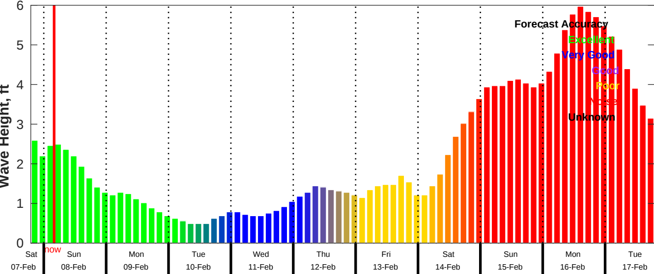
CMEMS Wave Forecast for NDBC 42040 from 07-Feb-2026 19:00:00 to 17-Feb-2026 19:00:00
