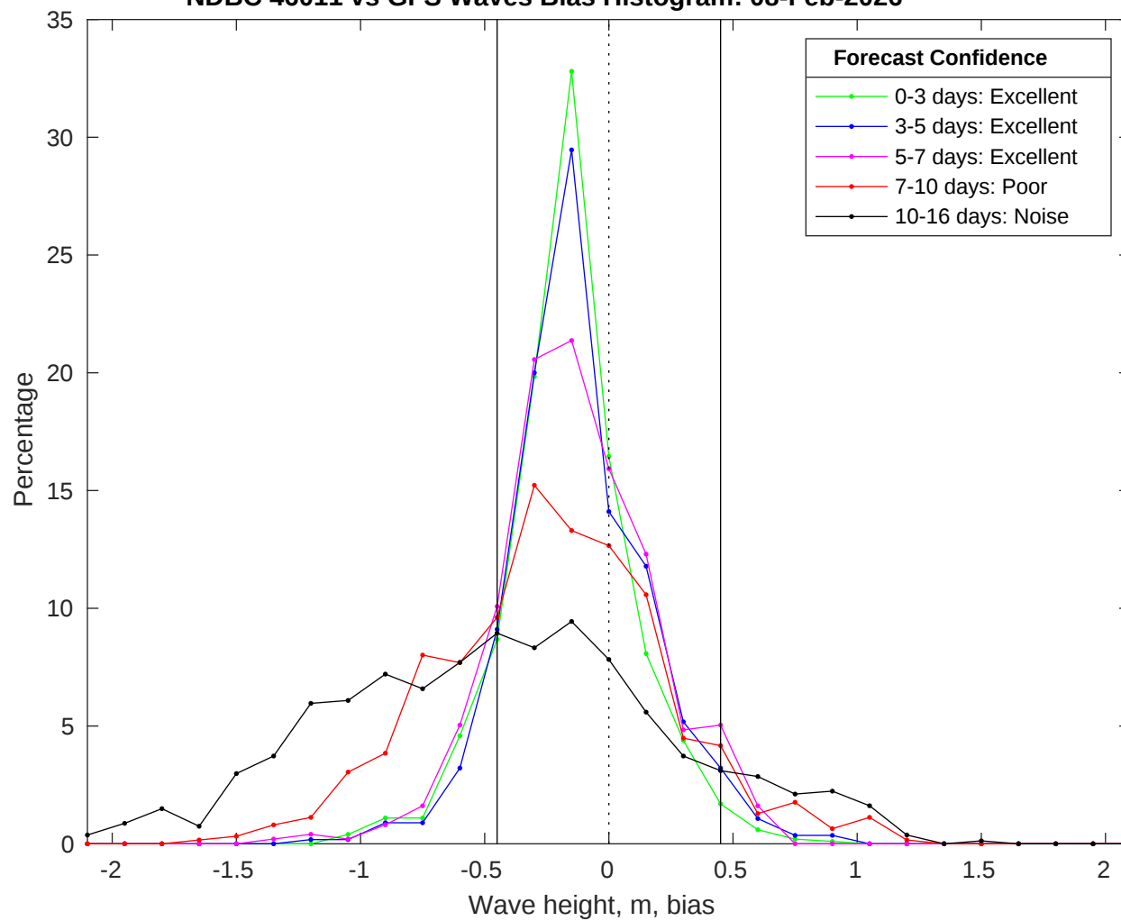
NDBC 46011 vs GFS Waves Bias Histogram: 08-Feb-2026
