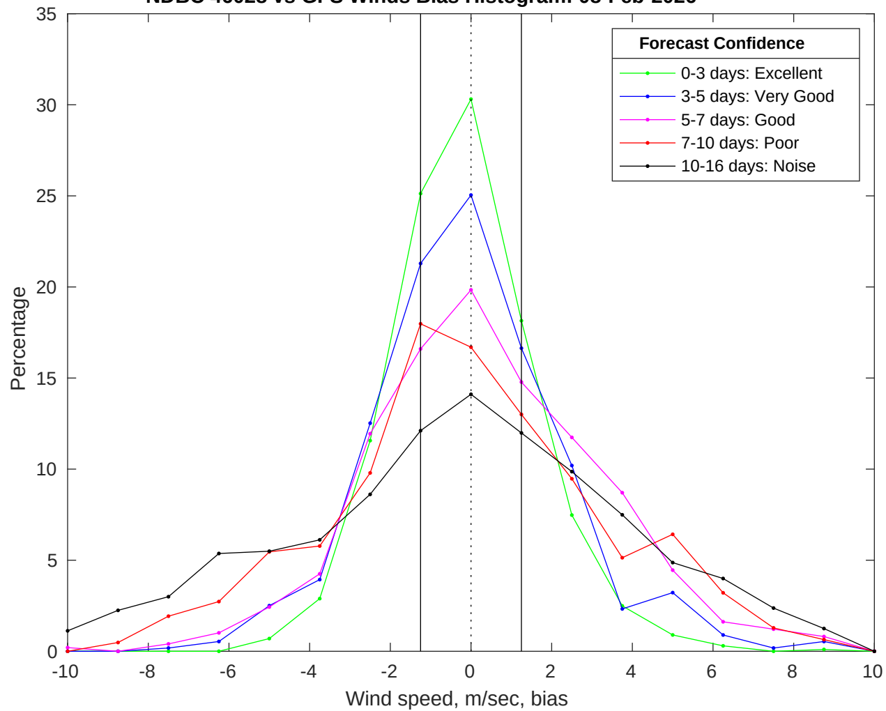
NDBC 46028 vs GFS Winds Bias Histogram: 08-Feb-2026
