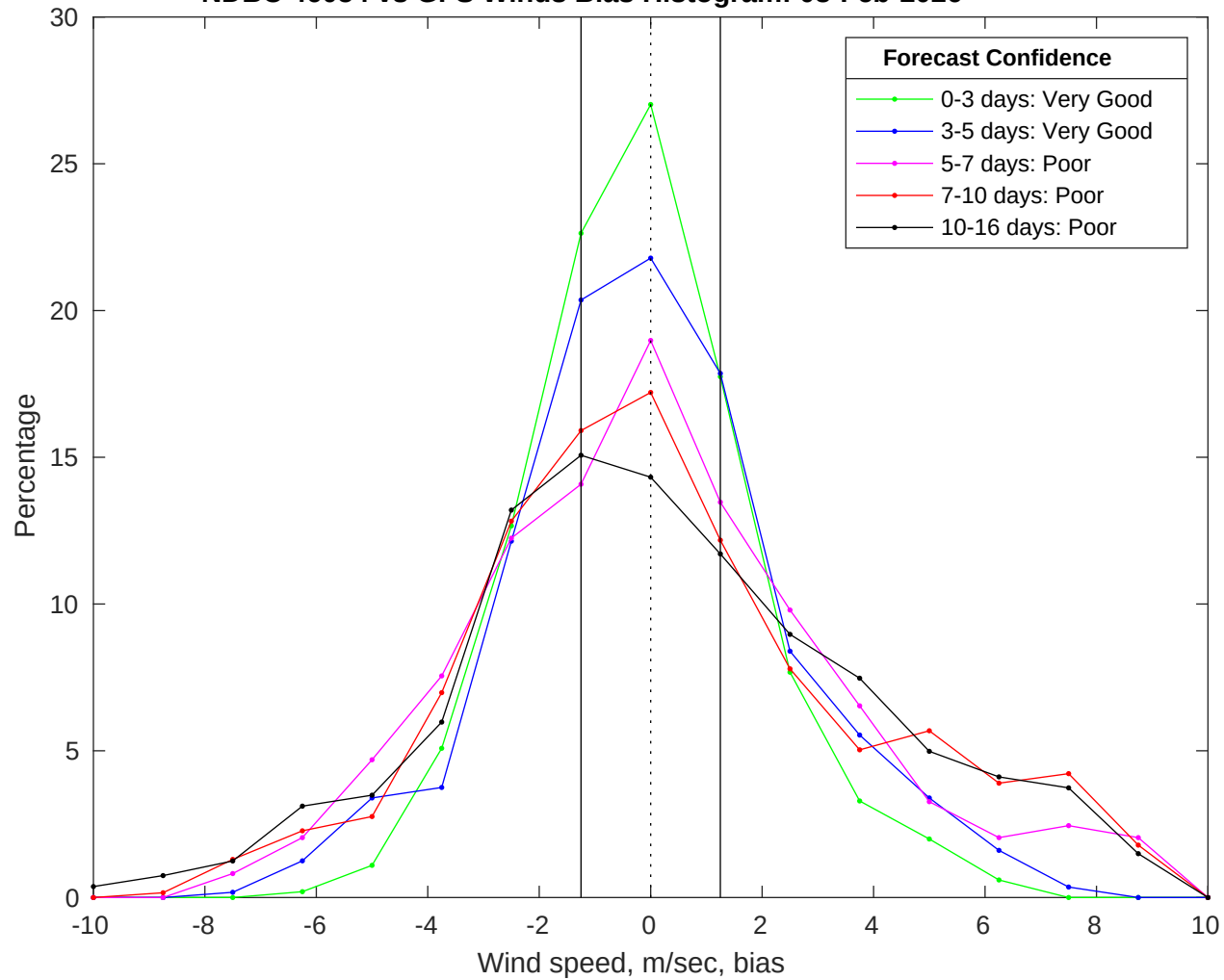
NDBC 46054 vs GFS Winds Bias Histogram: 08-Feb-2026
