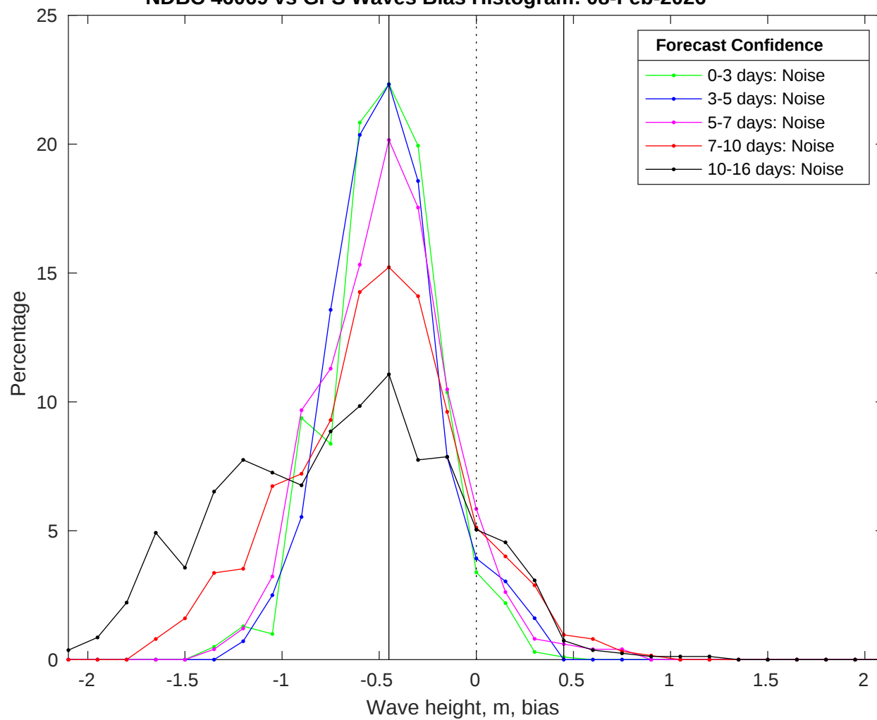
NDBC 46069 vs GFS Waves Bias Histogram: 08-Feb-2026
