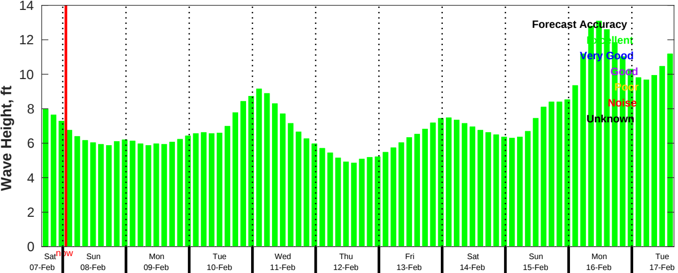
CMEMS Wave Forecast for NDBC 46215 from 07-Feb-2026 16:00:00 to 17-Feb-2026 16:00:00
