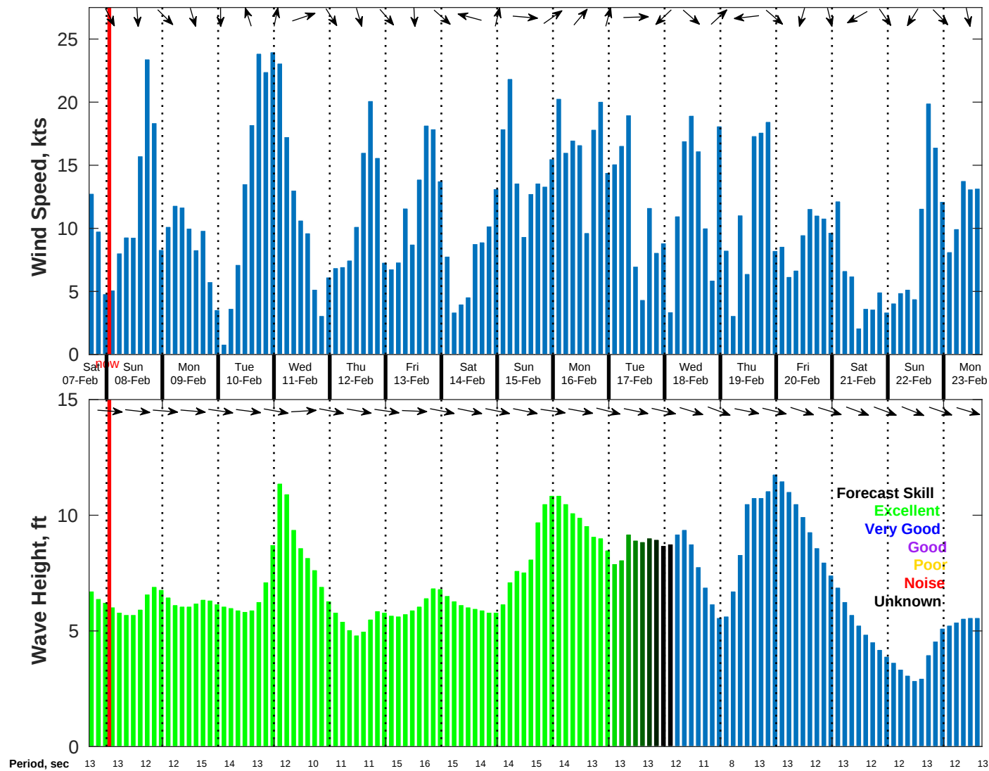
Wind & Wave Forecast for NDBC 46215 from 07-Feb-2026 16:00:00 to 23-Feb-2026 16:00:00
