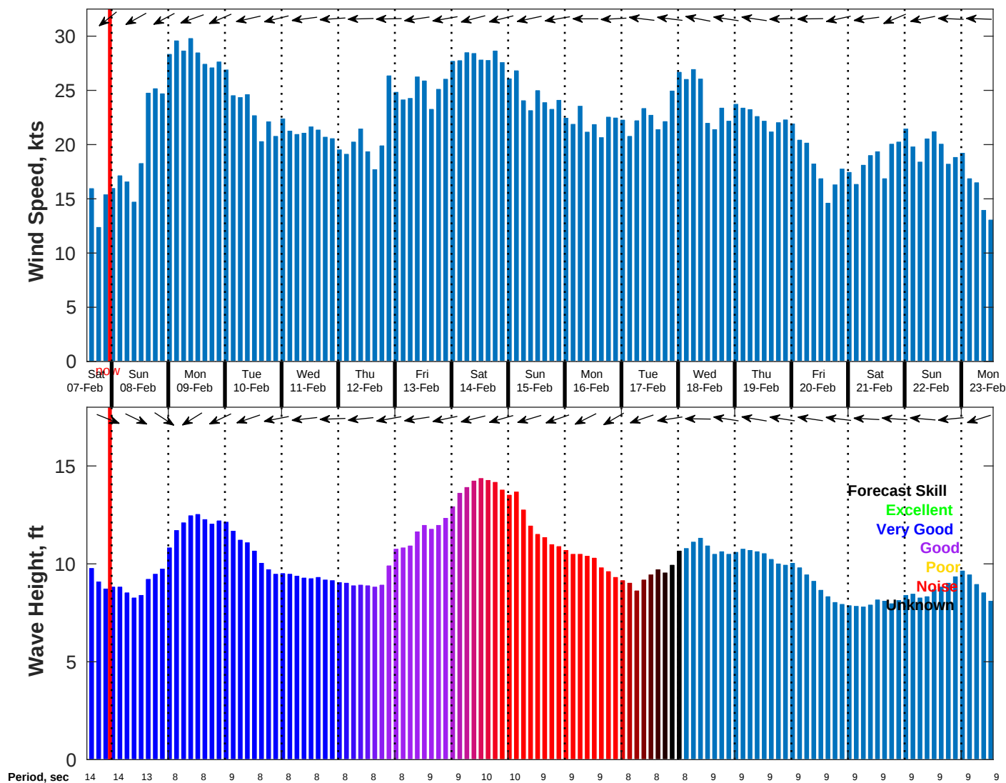
Wind & Wave Forecast for NDBC 51000 from 07-Feb-2026 14:00:00 to 23-Feb-2026 14:00:00
